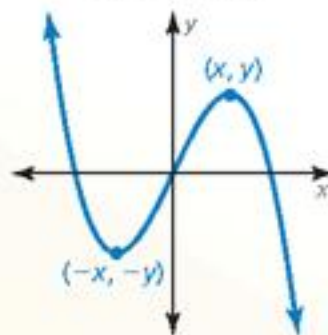
Odd Function
