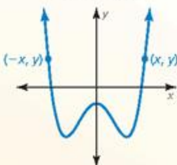
Even Function
