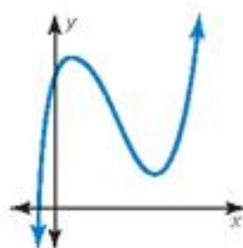
Graph of a continuous function
